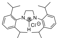
KP07-100002 1,3-Bis(2,6-diisopropylphenyl)-4,5-dihydroimidazolium chloride, ≥97.0% C_{27}H_{39}ClN_2 ; F.W: 427.06; [258278-25-0]
